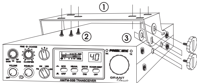
MOUNTING DIAGRAM
